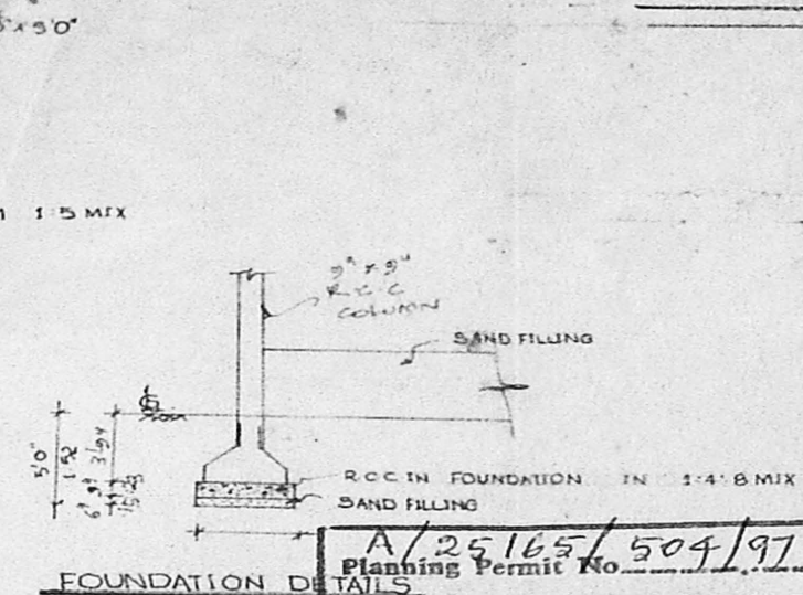
FOUNDATION DETAILS
