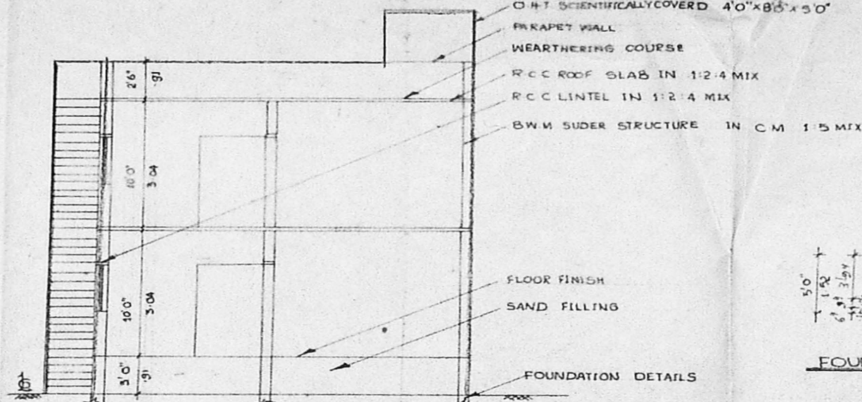
SECTION ON AA-BB
